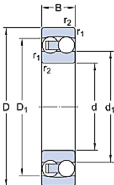
Cylindrical Bore
